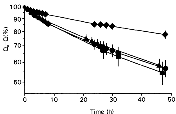
FIG. 2. Penetration of chloramphenicol from Eudragit RL lacquers containing different concentrations, C_L , of drug, through the hoof membrane at 32°C, plotted as the amount of drug remaining in the lacquer ( Q_0 - Q ; n=4 , mean \pm s.d.). Chloramphenicol concentration: ● 2.2%, ■ 18.5%, ▲ 31.3%, ◆ 47.6%.
